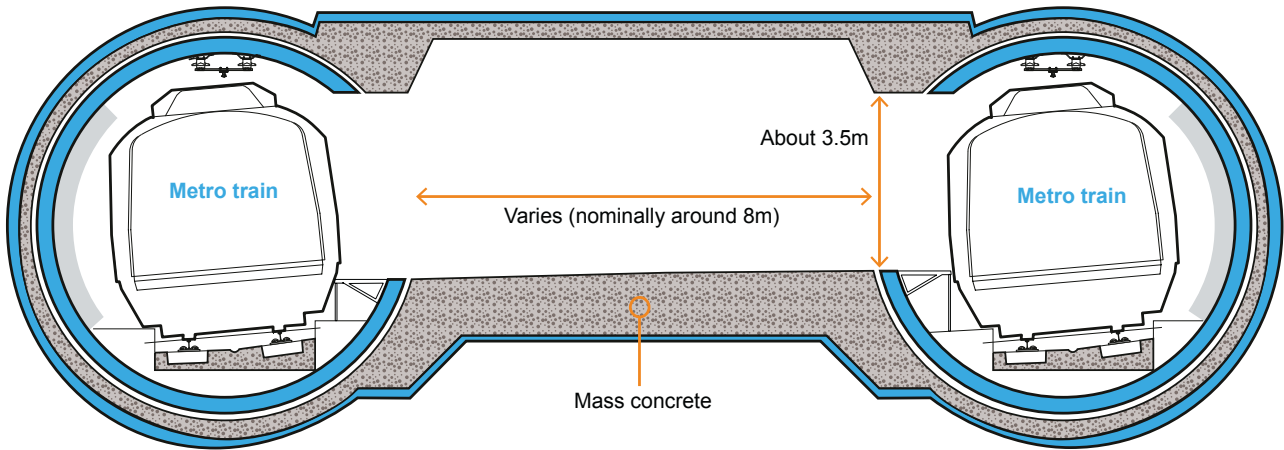
Indicative cross-section of a tunnel cross-passage
